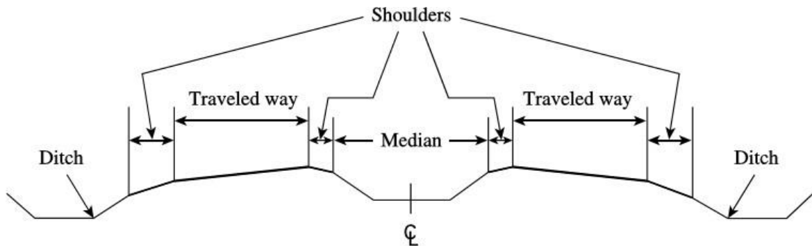
Fig.5.2. Divided highway cross section, depressed median, with ditches.
