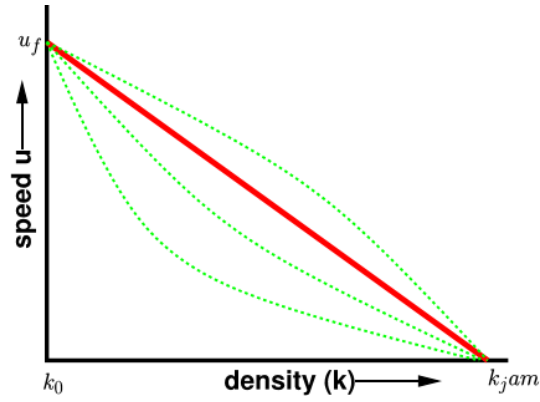
Fig.13.2 Speed-density diagram
