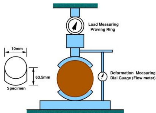
Fig. 30.1 Marshall Mould
