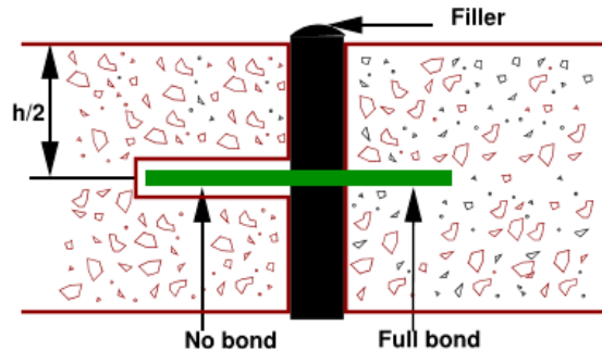
Fig. 35.1 Expansion joint
