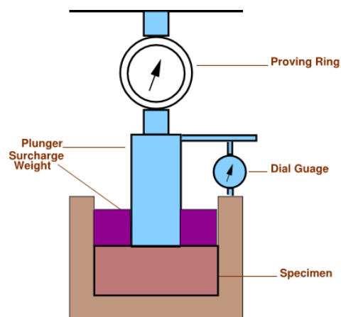
Fig 21.1 CBR Test
