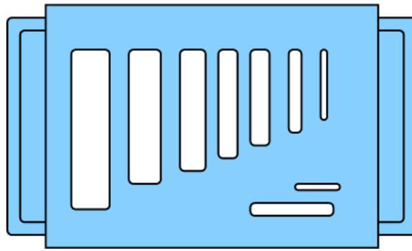
Fig.24.1 Flakiness gauge
