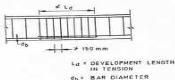
FIG. 2 LAP SPLICING IN BEAM
