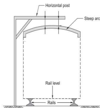
Fig. 2.2 Loading gauge
