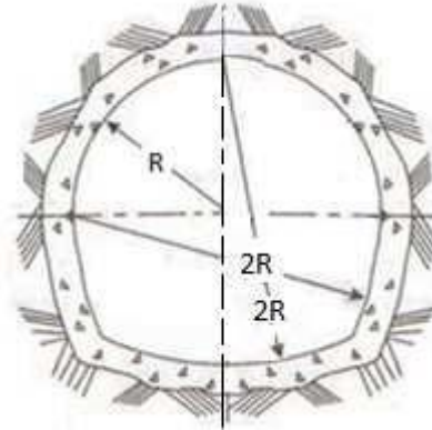
Figure 18.4 Horse-Shoe Section
