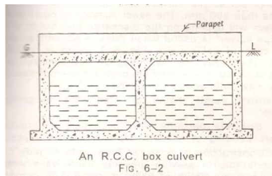
Fig. 6-2 shows an R.C.C box culvert with two openings. Following points should be noted.
