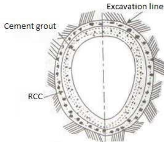
Figure 18.6 Egg-shaped Section
