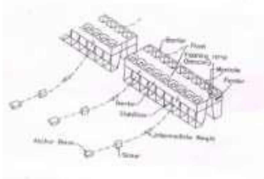
Fig. 14.3. Schematic diagram of floating breakwater
