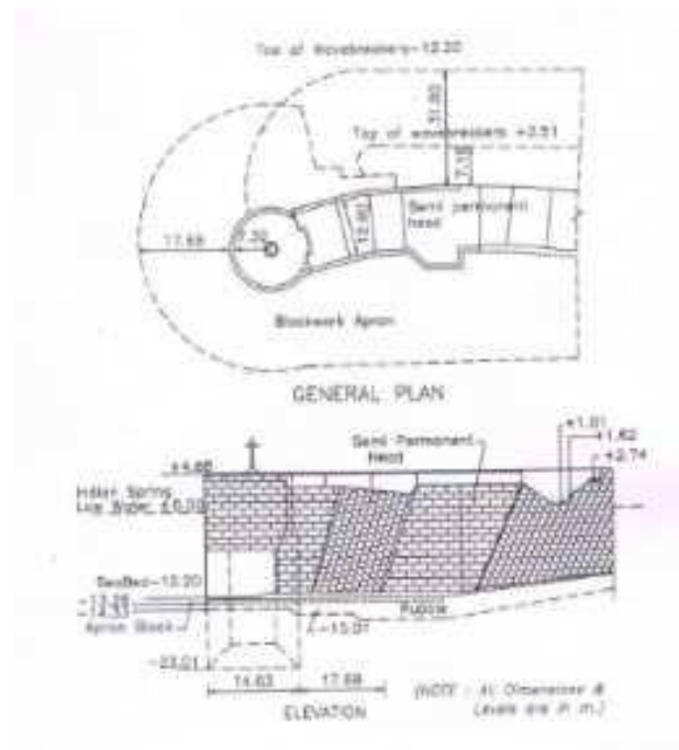
Fig.14.1 Vertical Breakwater wall at Madras
