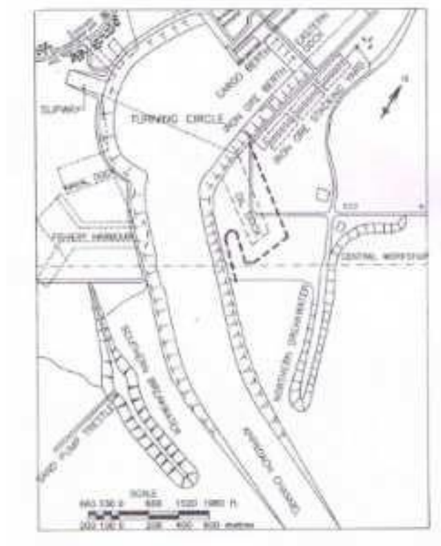
Fig. 13.2 Layout of ParadipHarbour
