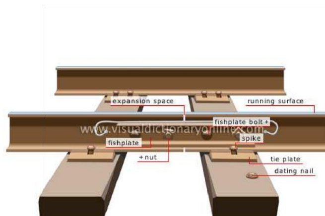
The first railway fishplate
