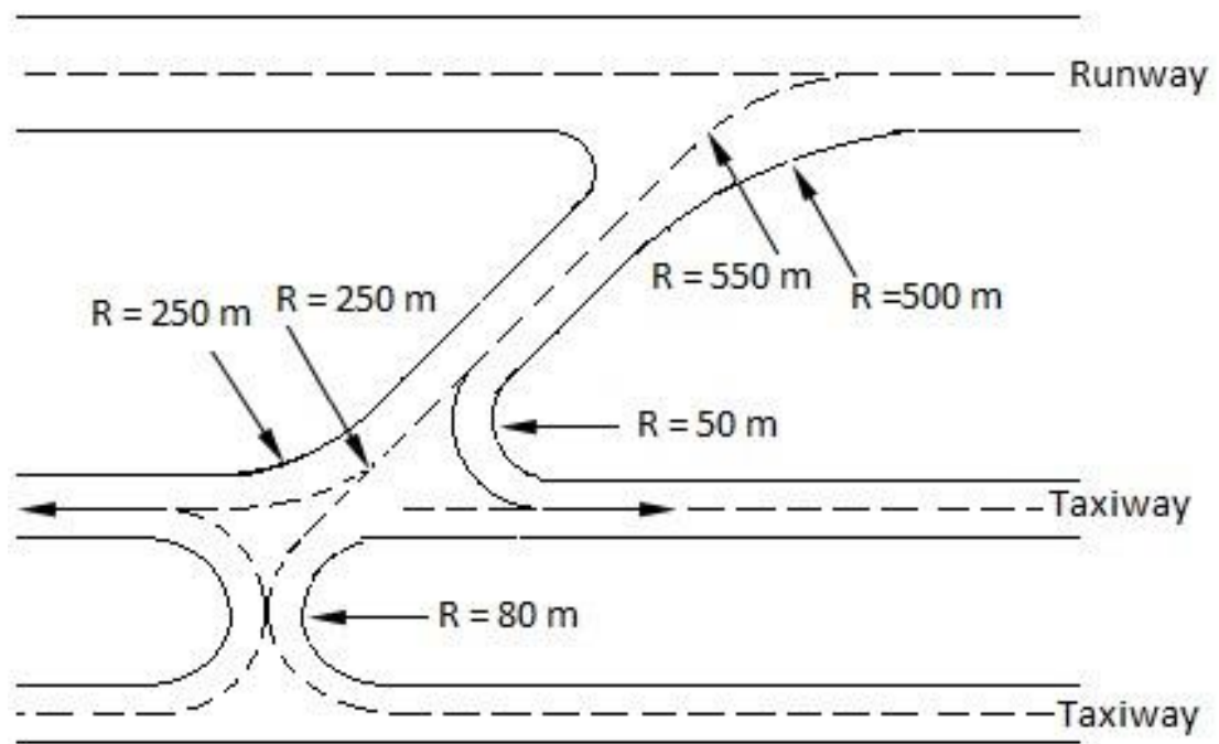
Figure 17.2 Runway and Taxiway Exit Details
