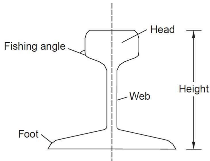
Flat-footed rail
