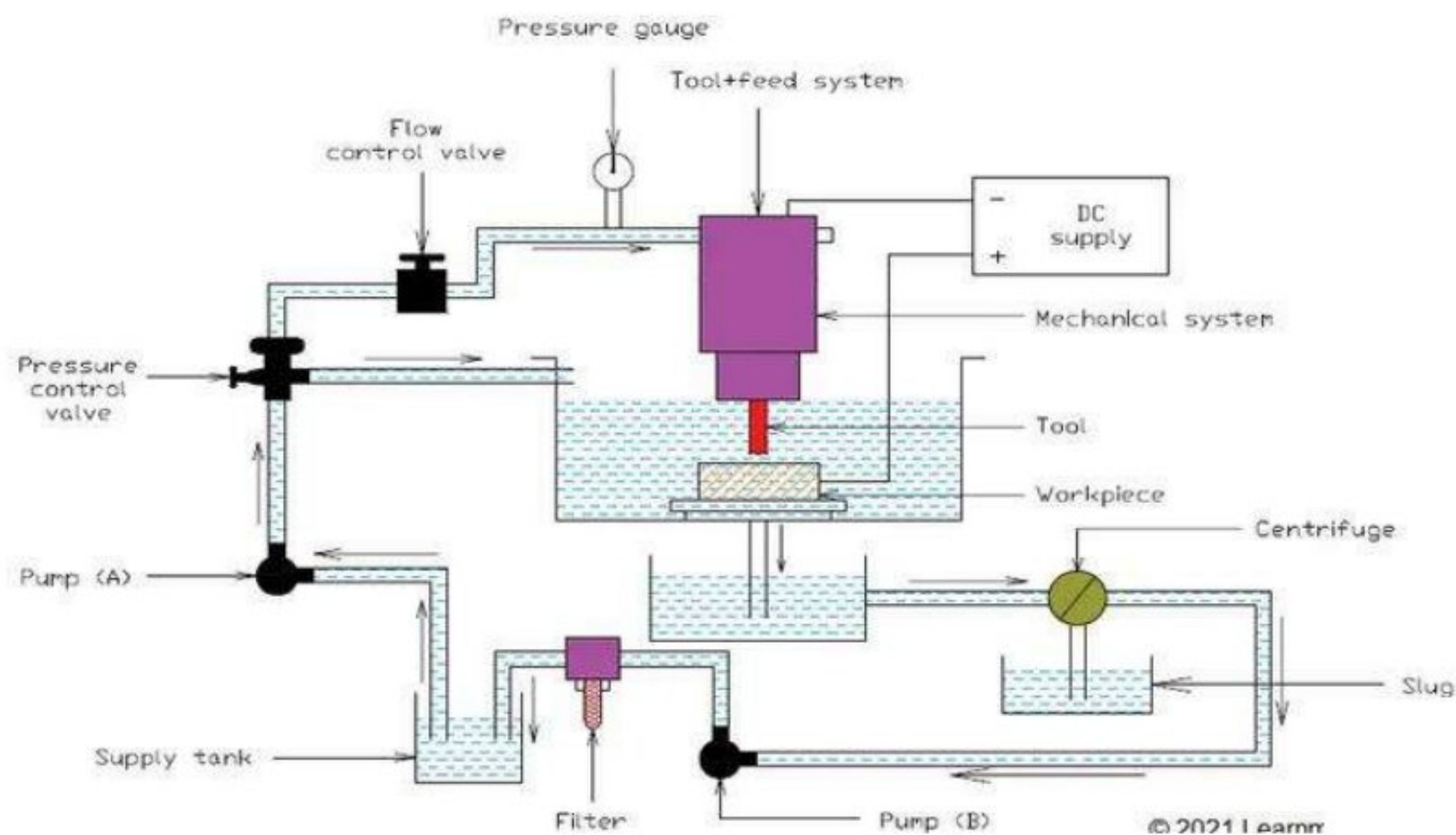
Diagram of Electro-Chemical Machining Setup
