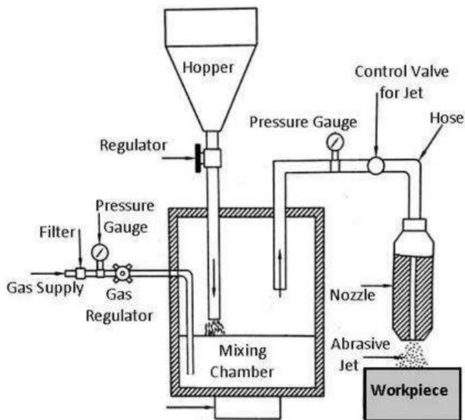
Principle of Abrasive Jet Machining
