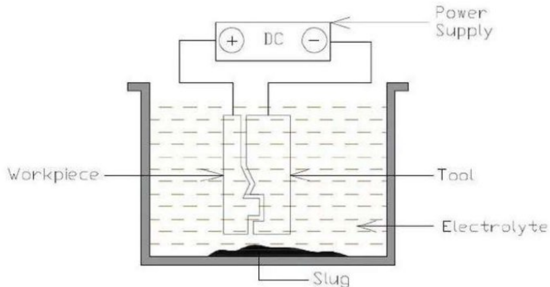
Diagram of Conceptual Electrochemical Model,
