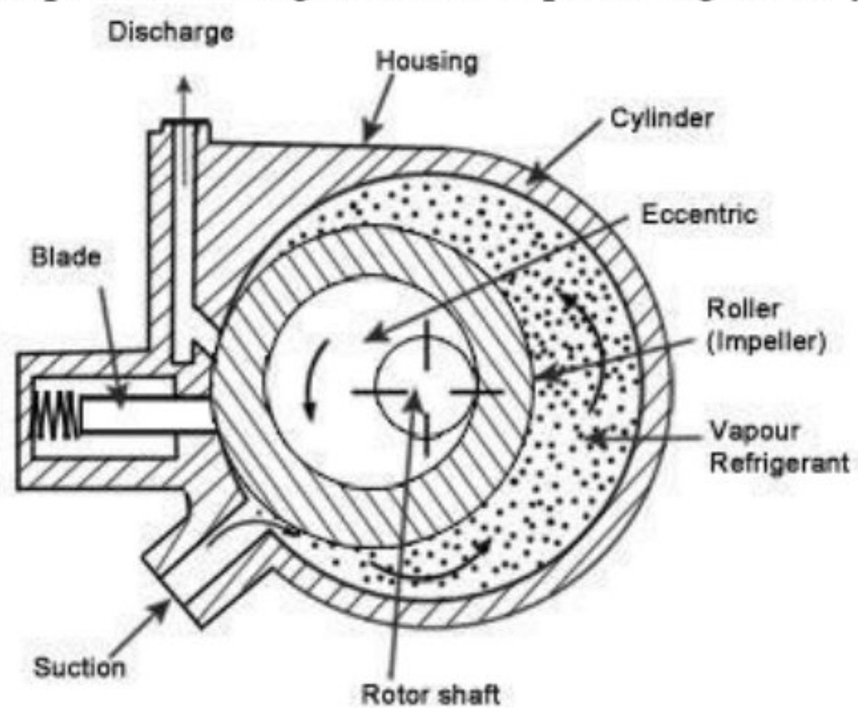
(a) Completion of intake stroke and beginning of compression
