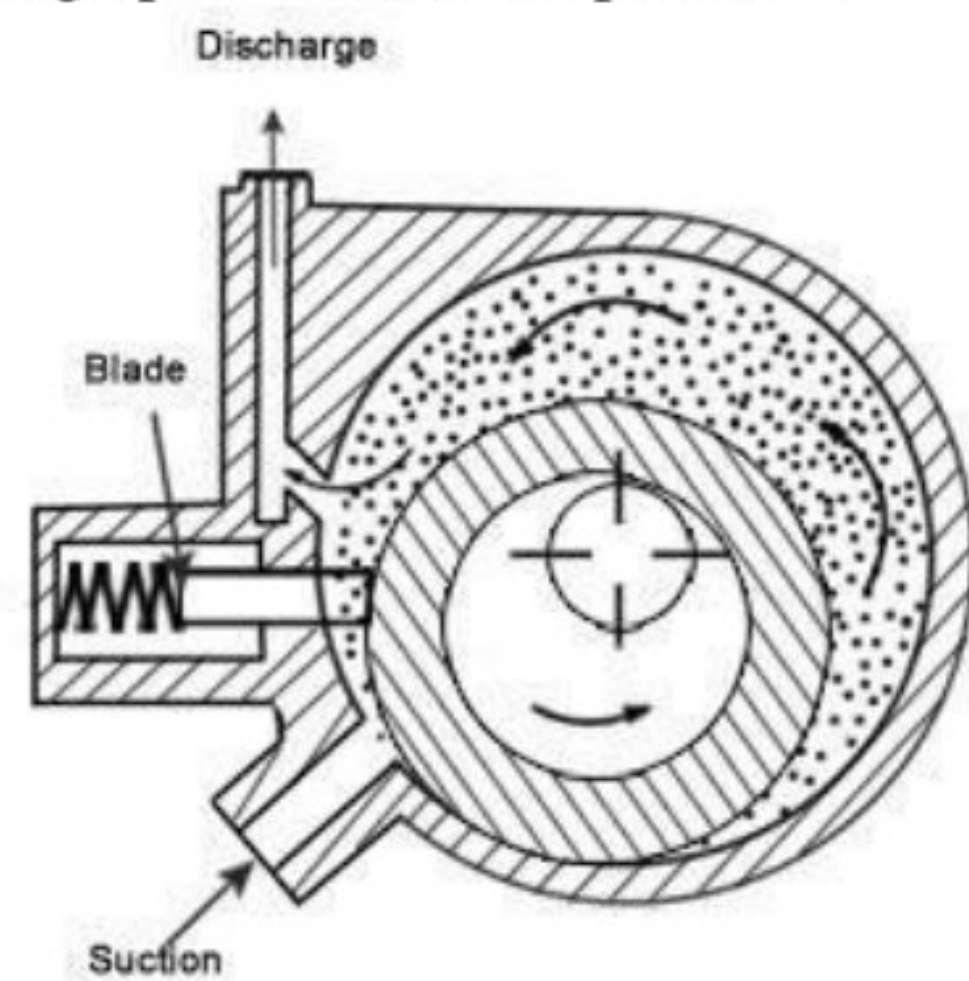
(b) Compression stroke continued and new intake stroke started
