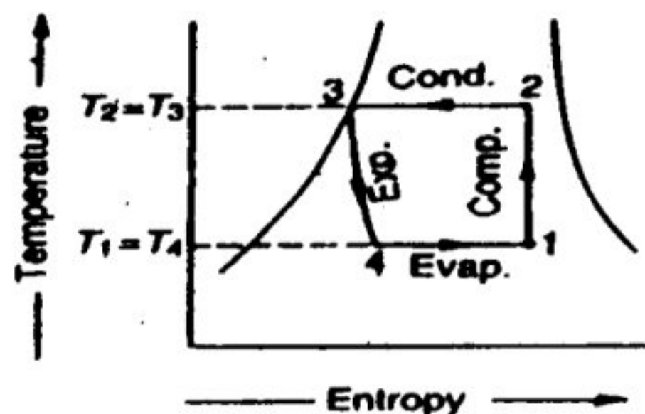
(a) T-s diagram.
