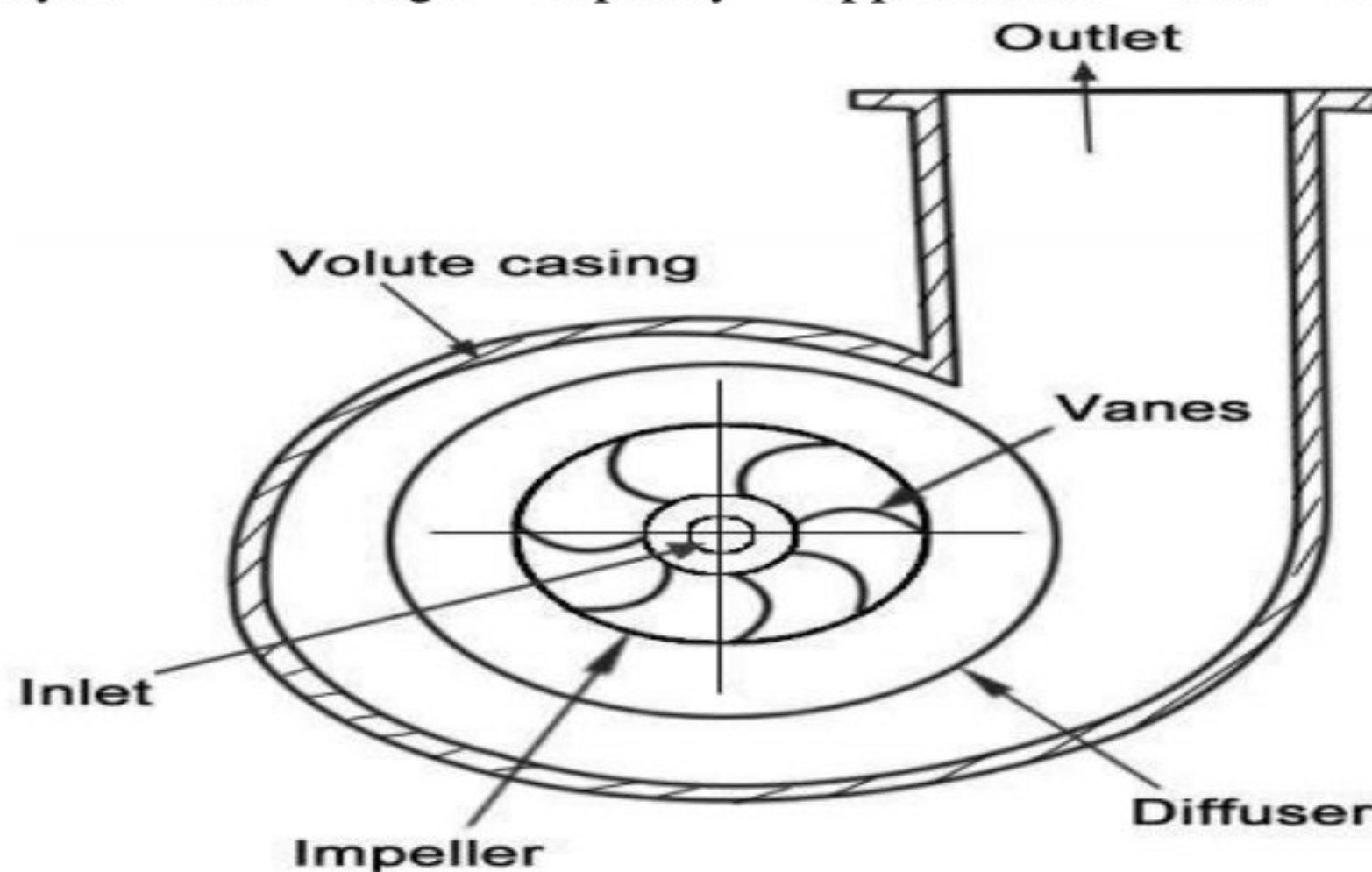
Centrifugal compressor
