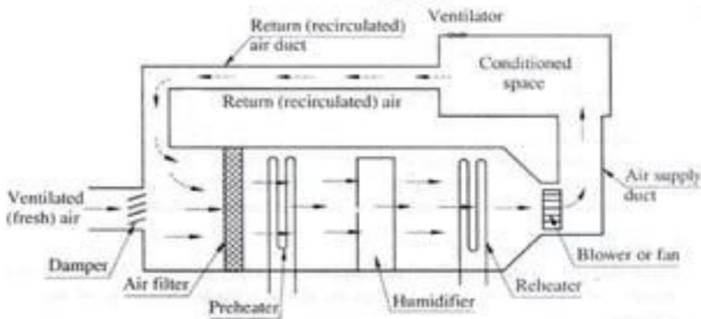
Fig. Winter air conditioning system
