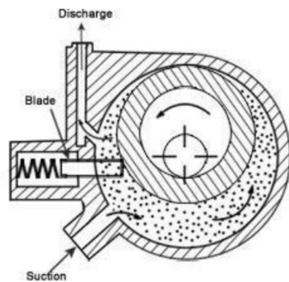
(d) Compressor vapour discharged to condensor and new intake stroke continued
