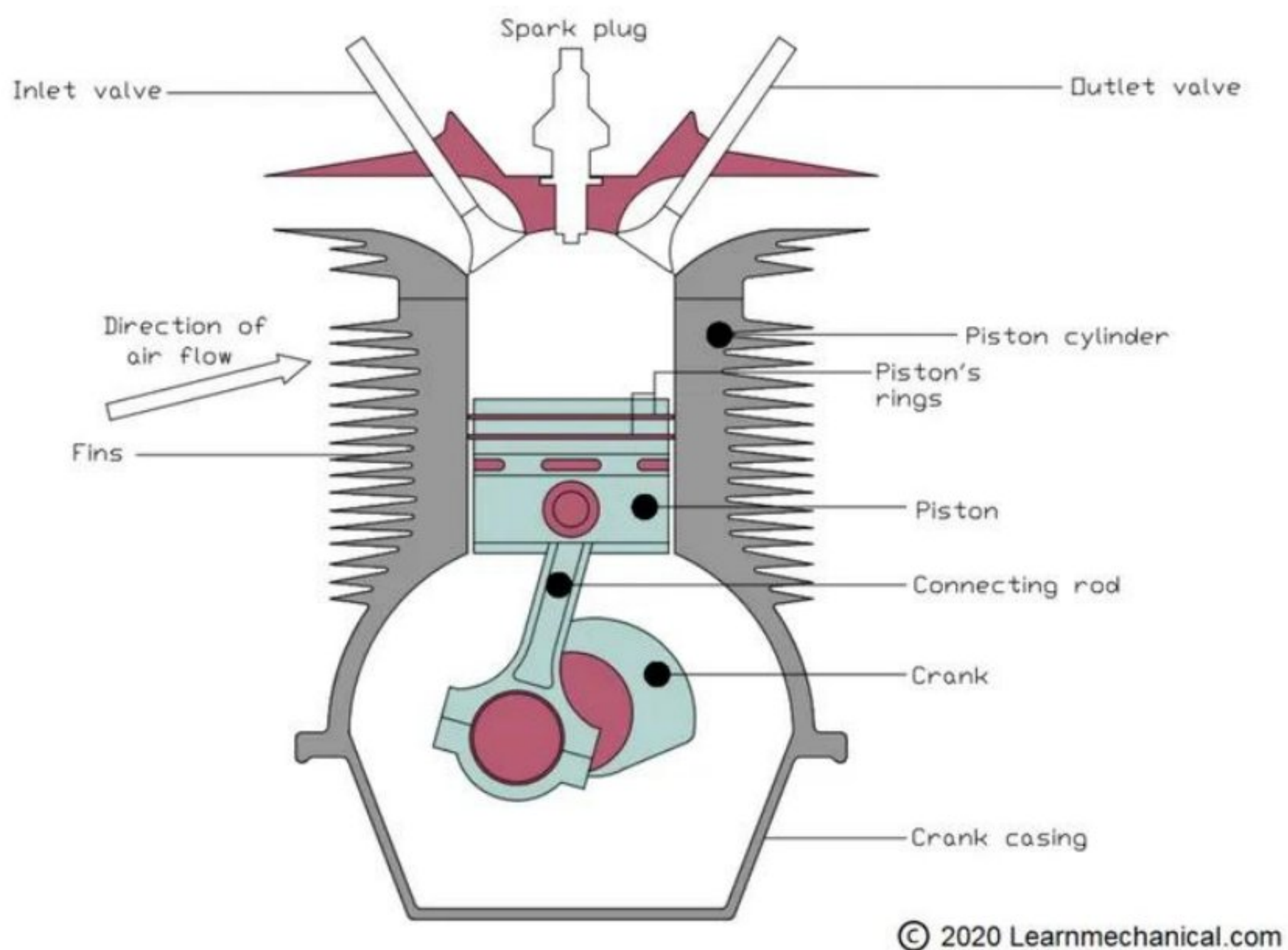
Air-Cooling System
