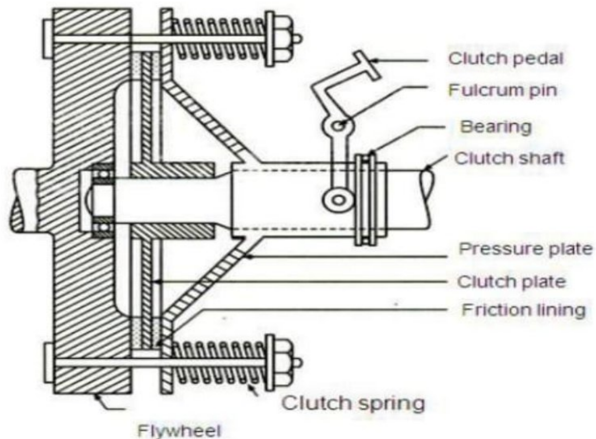
Figure: Single Plate Dry Clutch
