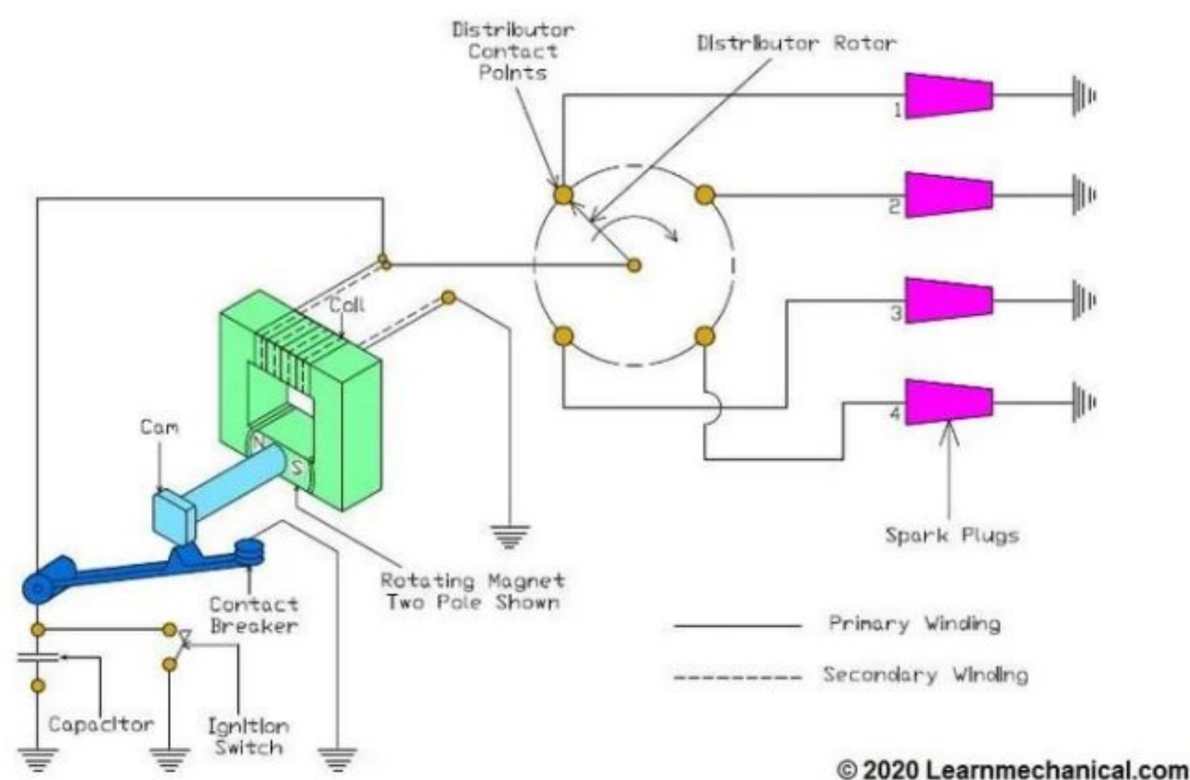
Magneto Ignition System
