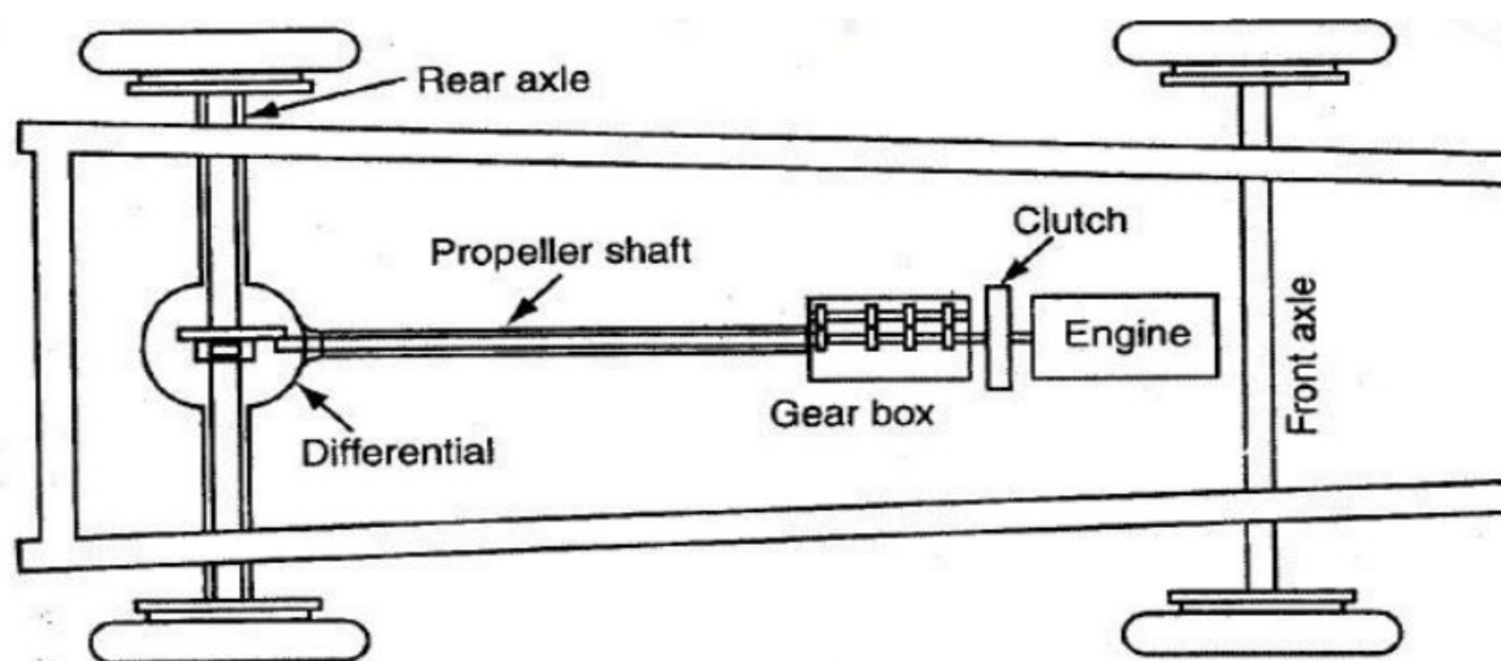
General arrangement of power transmission
