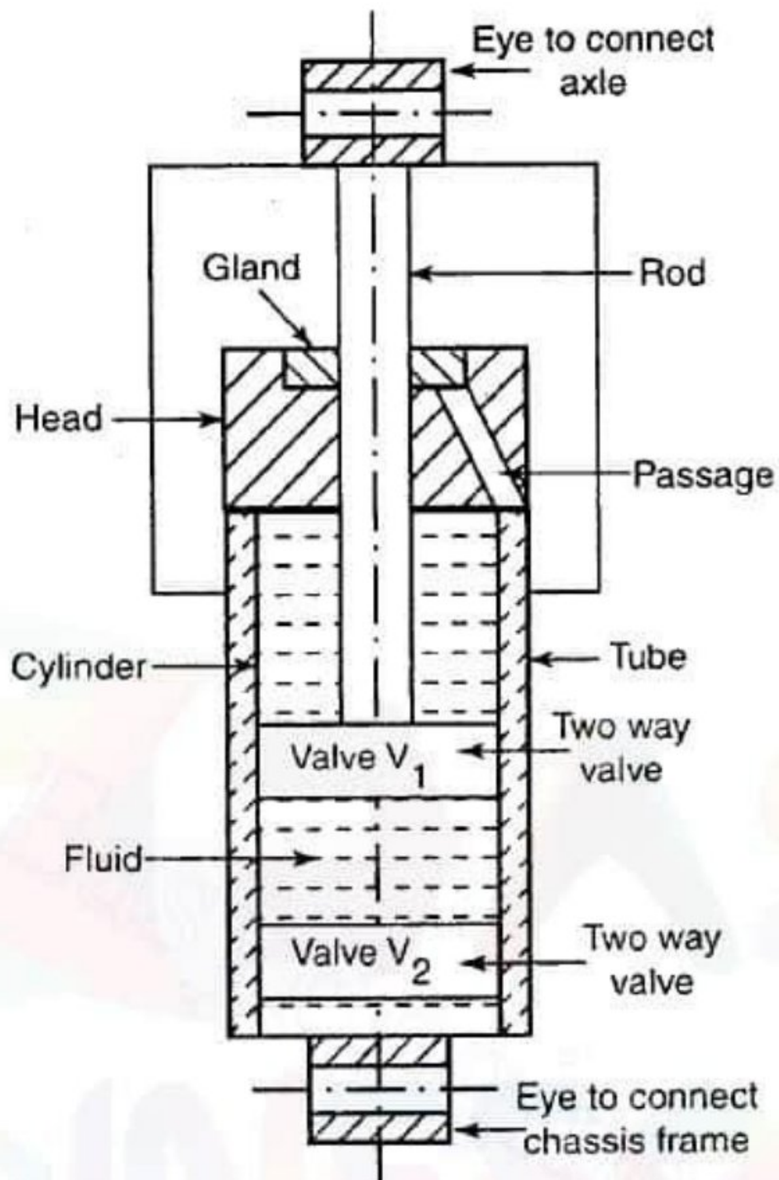
Figure 4.55 Telescopic shock absorber
