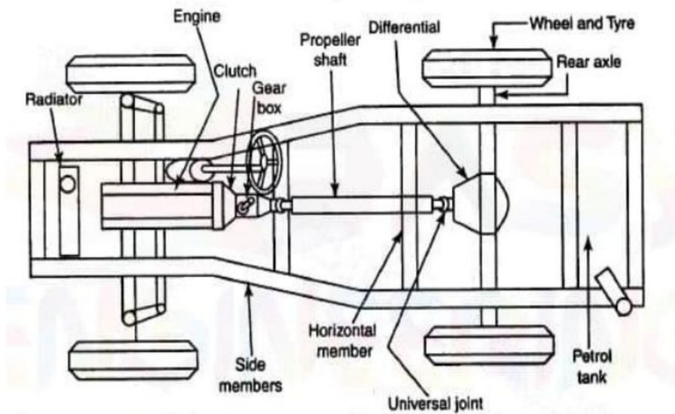
Top view (Plan)
