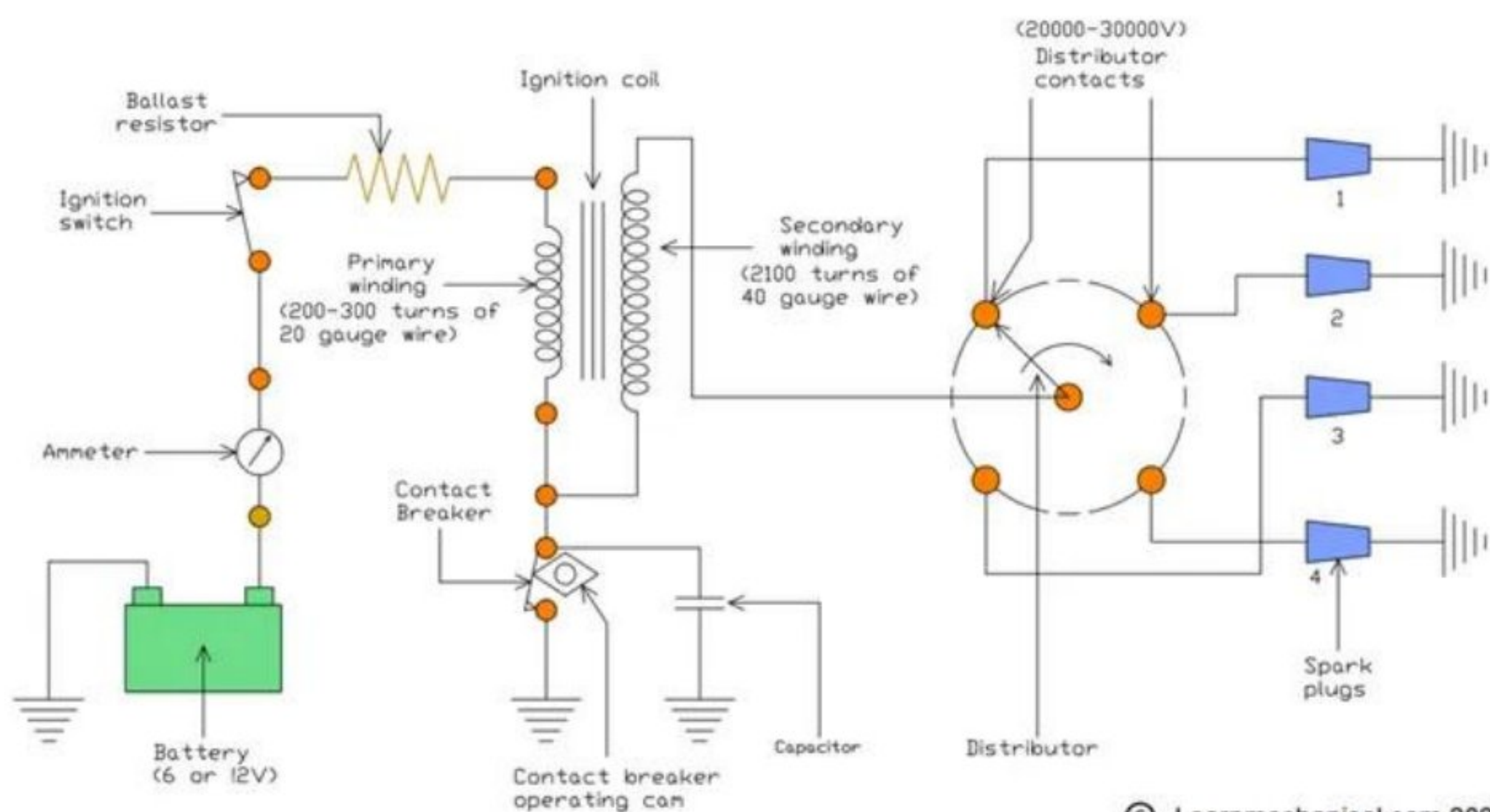
Diagram of Battery Ignition System, Learn Mechanical
