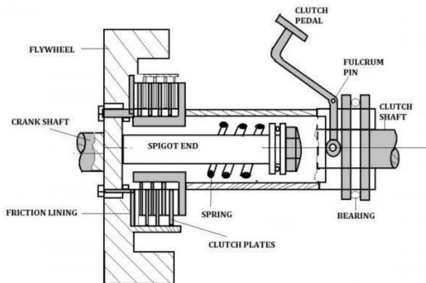
FIG: MULTI PLATE CLUTCH
