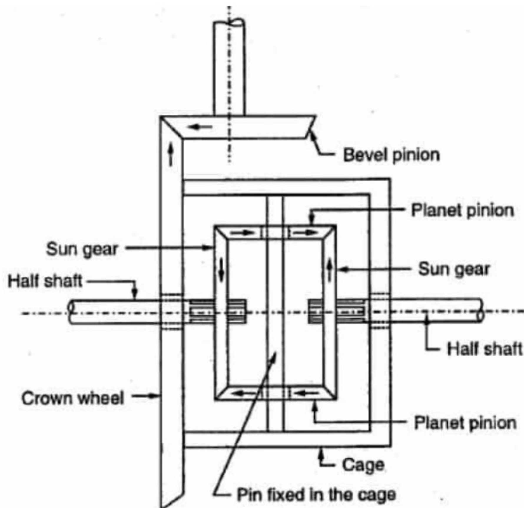
Figure: Working of differential
