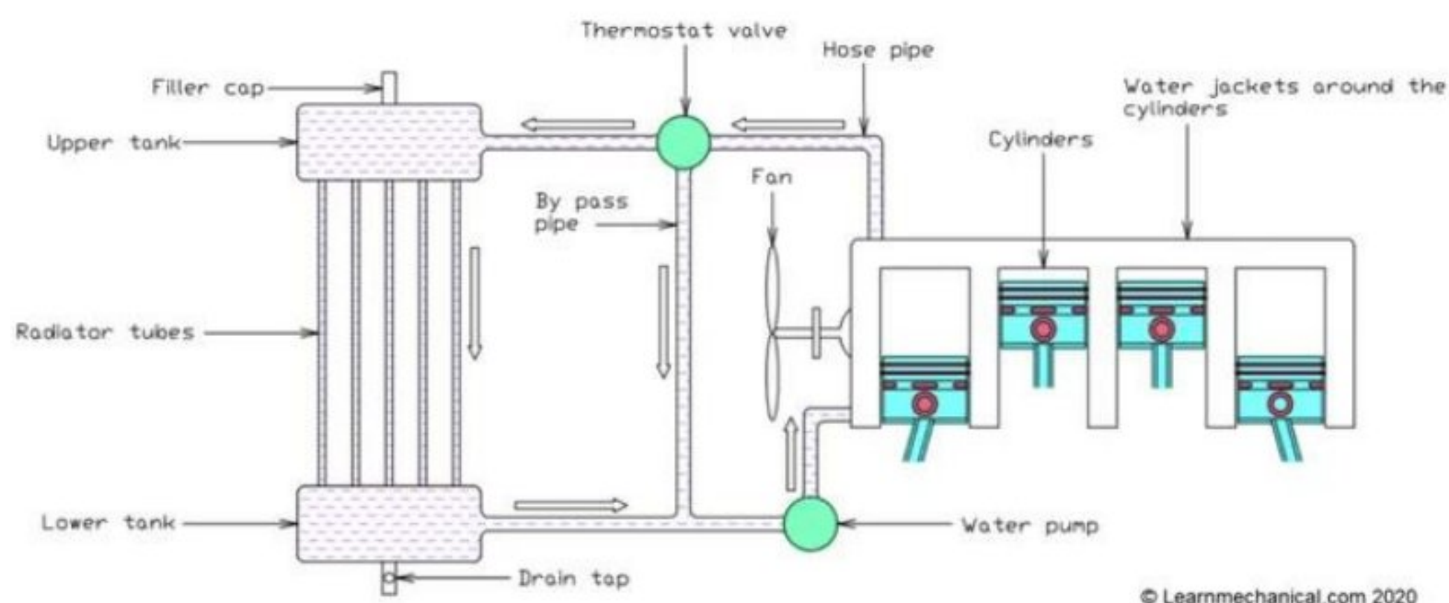
Parts of Water Cooling System
