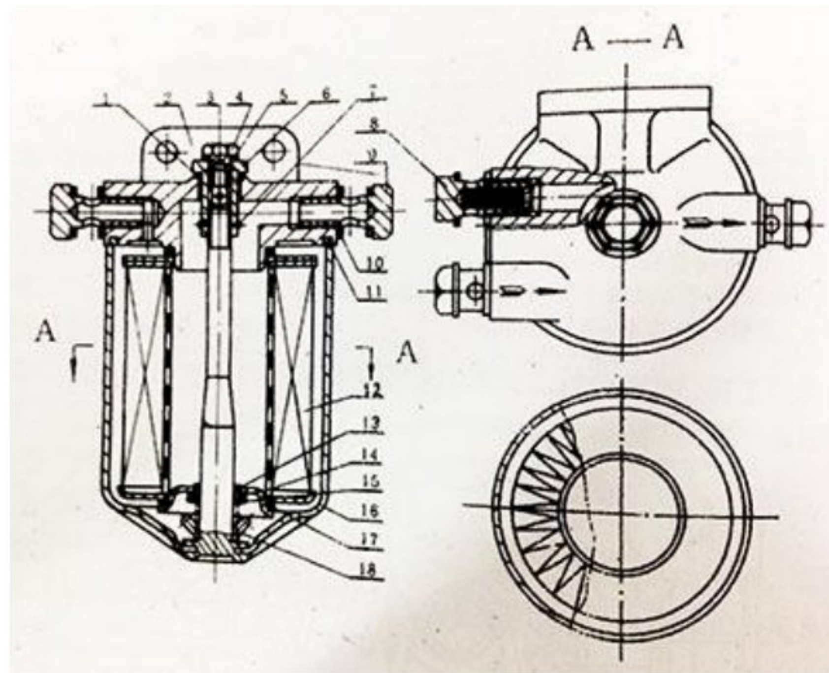
Figure 1: Fuel filter assembly section
