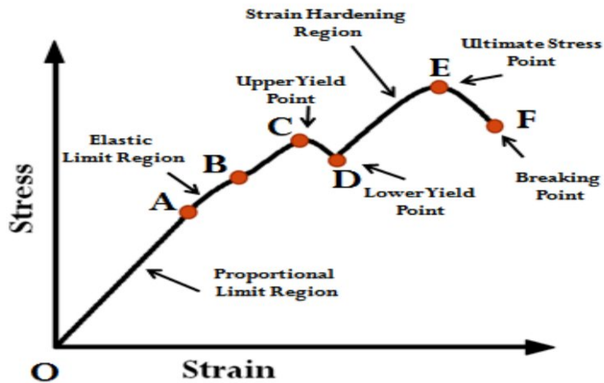
Fig.Stress-strain curve for mild steel
