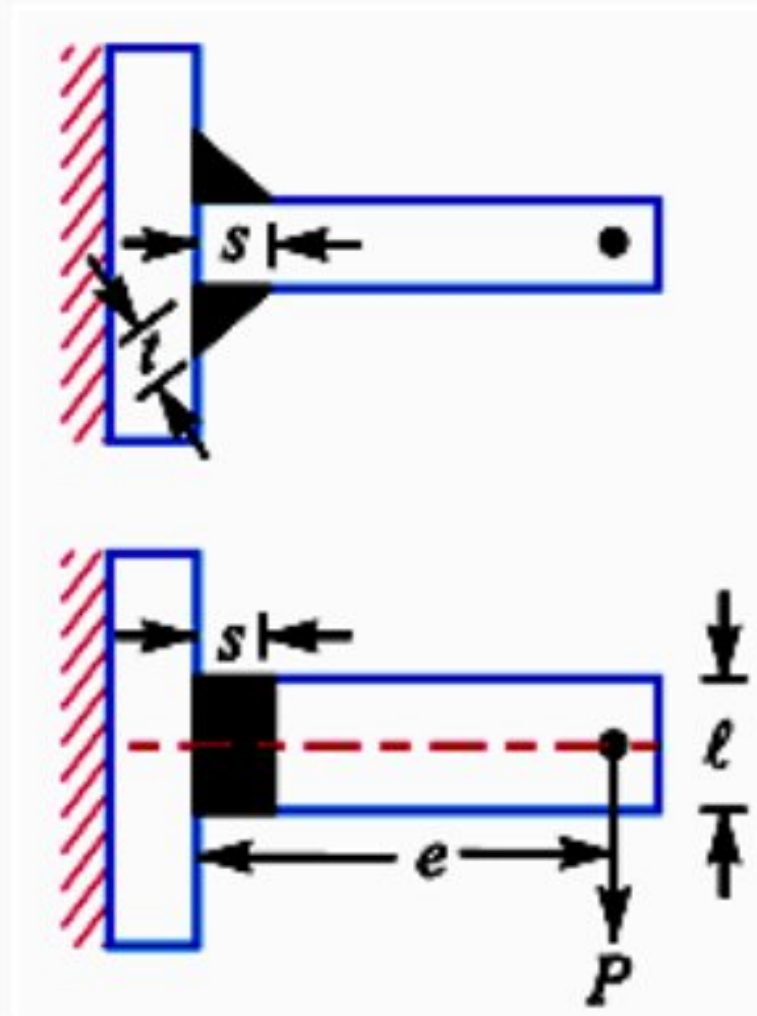
Figure. Bending Stress due to Eccentricity
