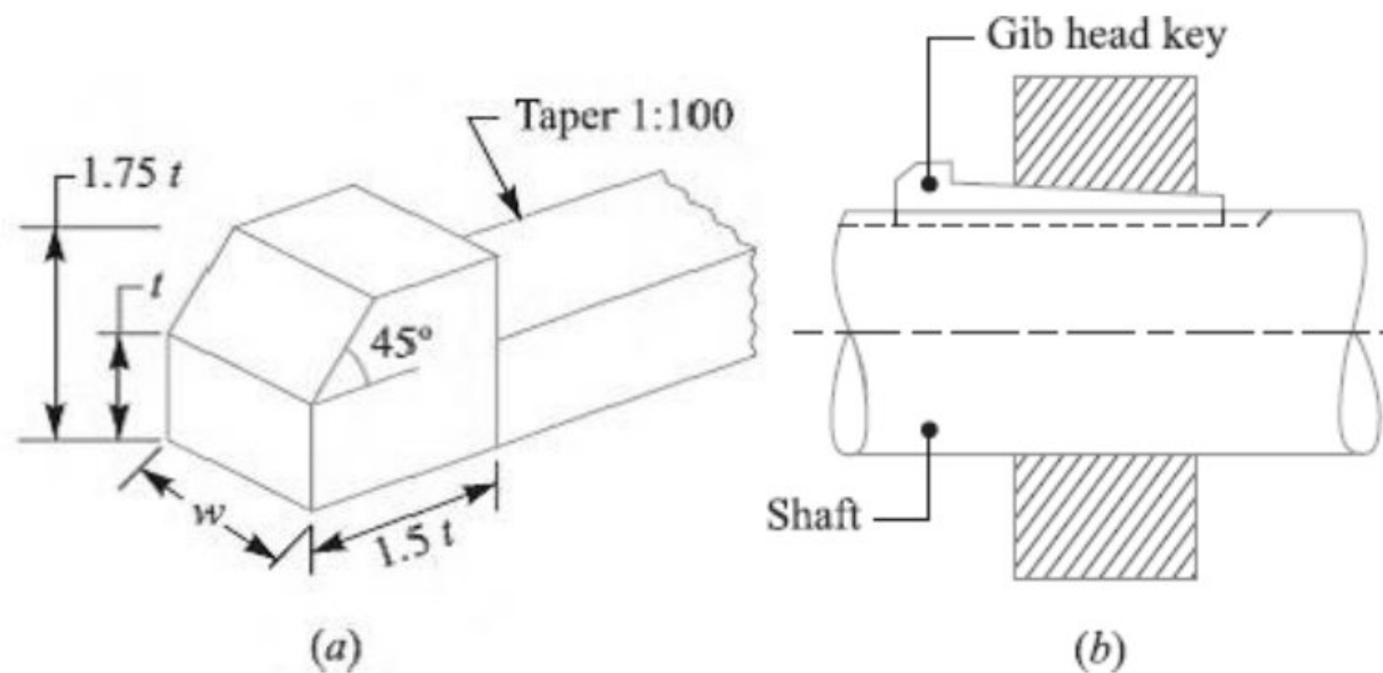
Fig. Gib head key and its use
