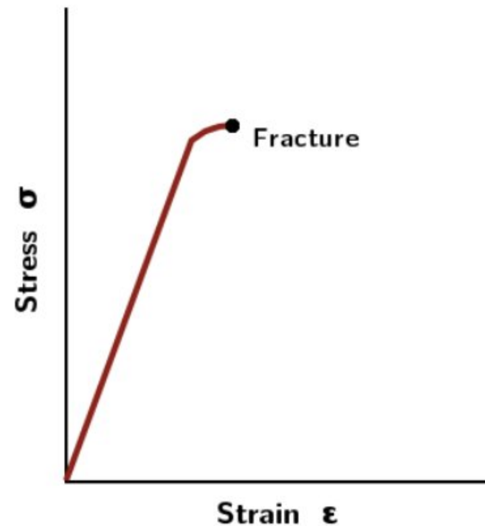
Fig. stress-strain curve for cast iron.
