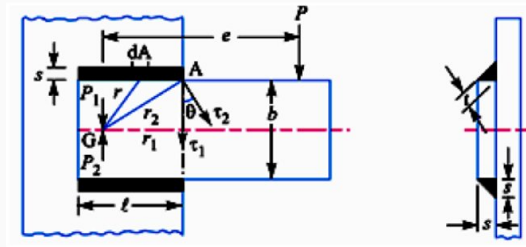
Figure. Shear Stress due to Eccentricity
