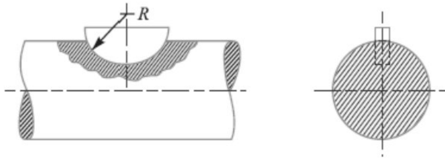
Fig. Woodruff Key
