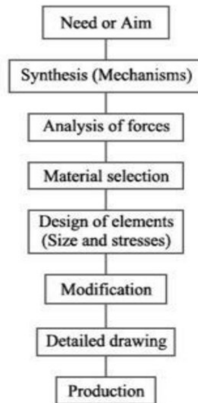
Fig. General Machine Design Procedure
