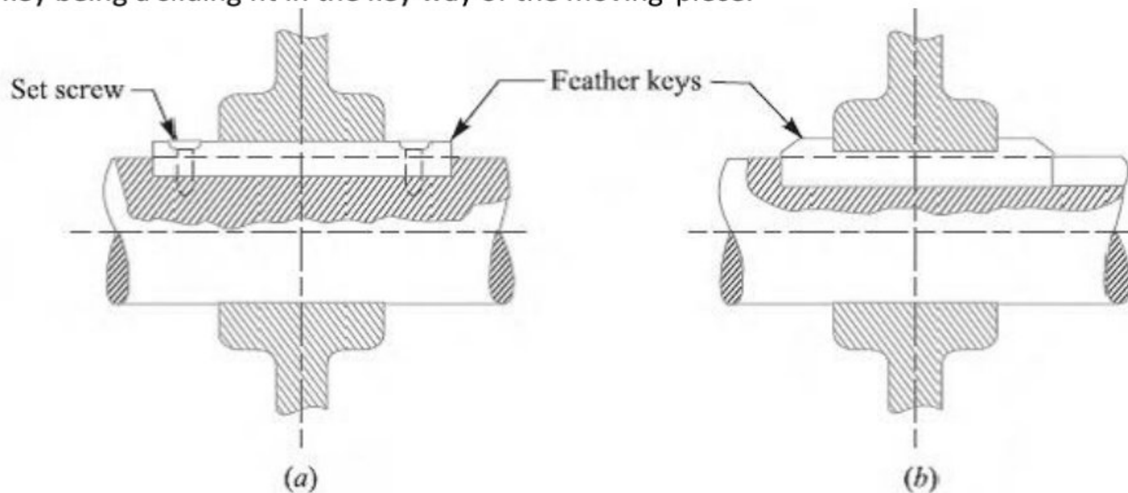
Fig. Feather Keys
