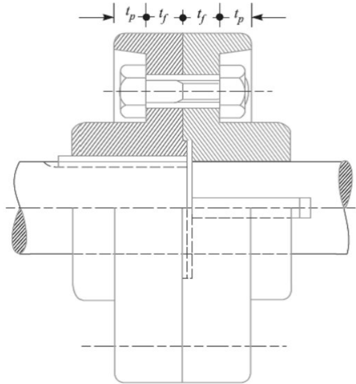
Fig.2. Protected Type Flange Coupling.
