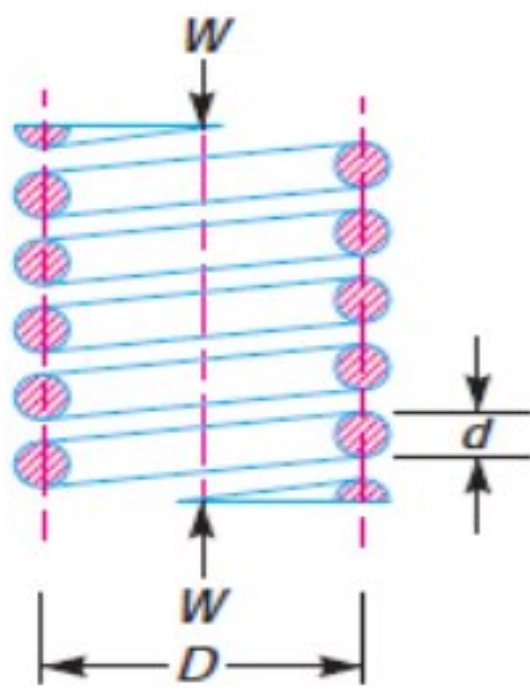
(a) Axially loaded helical spring.
